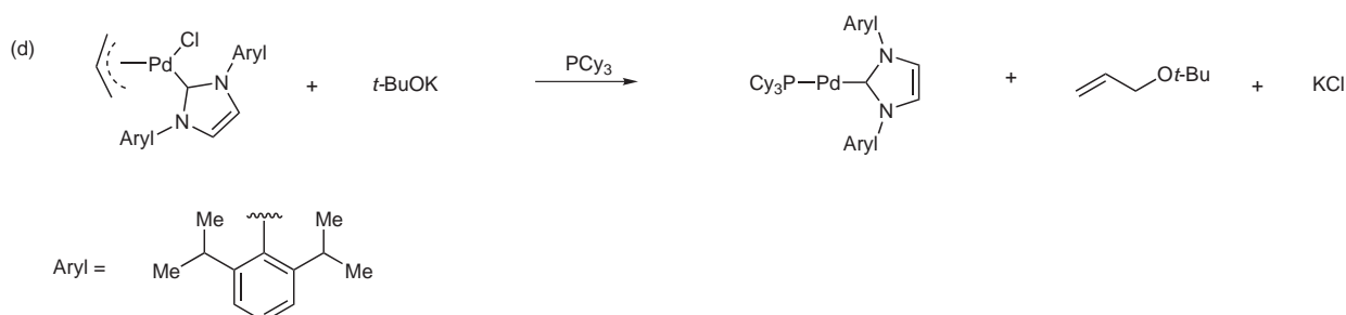
Scheme 1 Reduction pathways of Pd(II) sources: reduction by formation of (a) and (b) phosphine oxides, (c) aldehyde from imine, (d) tert -butyl allyl ether
