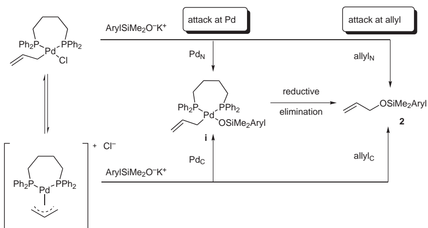
Scheme 3 Possible reductive pathways to form allyloxysilanes
