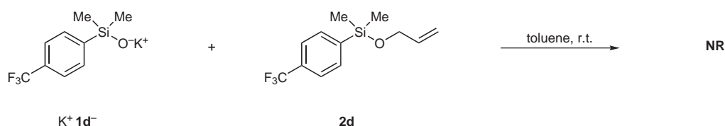
Scheme 4 Control experiment to probe formation of disiloxane from 2d
