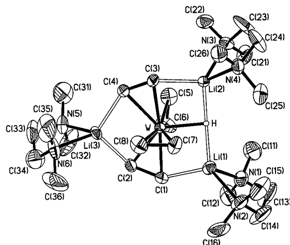
Figure 1. Molecular structure of [\text{Li}(\text{tmed})]_3[\text{WH}(\text{C}_2\text{H}_4)_4] , 1 . Thermal ellipsoids are represented by the 30% probability surfaces except for the hydride atom, which is represented by an arbitrarily sized sphere. Selected bond distances (Å) and angles (deg): W–C(1) 2.244(8), W–C(2) 2.208(7), W–C(3) 2.229(7), W–C(4) 2.233(7), W–C(5) 2.221(9), W–C(6) 2.233(8), W–C(7) 2.197(8), W–C(8) 2.182(8), W–Cn(12) 2.103(7), W–Cn(34) 2.107(7), W–Cn(56) 2.121(8), W–Cn(78) 2.067(8), W–H 2.04(5), C(1)–C(2) 1.463(10), C(3)–C(4) 1.466(10), C(5)–C(6) 1.357(11), C(7)–C(8) 1.447(11), Li(1)···H 1.945(55), Li(2)···H 1.991(54), Cn(12)–W–Cn(34) 137.6°, Cn(12)–W–Cn(56) 96.0°, Cn(12)–W–Cn(78) 87.8°, Cn(34)–W–Cn(56) 93.9°, Cn(34)–W–Cn(78) 87.0°, Cn(56)–W–Cn(78) 173.2°, Cn(12)–W–H 108.1°, Cn(34)–W–H 114.0°, Cn(56)–W–H 69.5°, Cn(78)–W–H 104.0°, where Cn represents the centroid of an ethene ligand.
