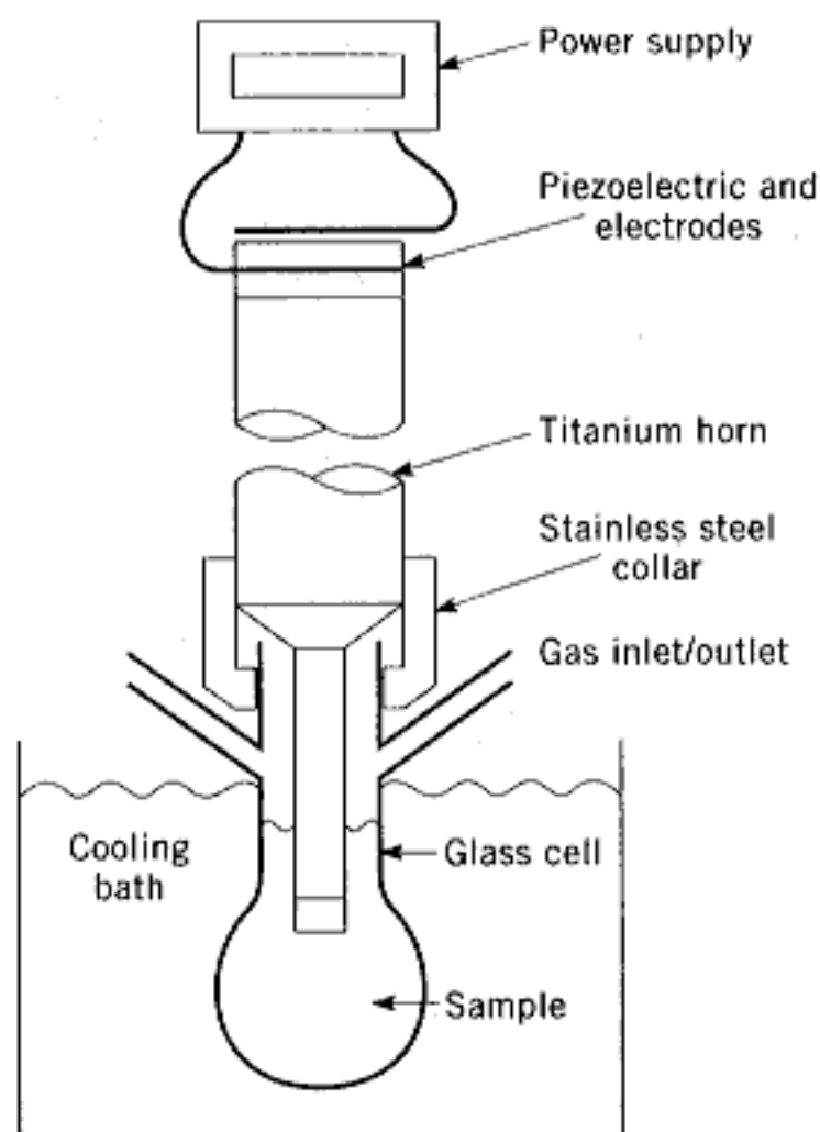
Fig. 9. A typical sonochemical apparatus with direct immersion ultrasonic horn. Ultrasound can be easily introduced into a chemical reaction with good control of temperature and ambient atmosphere. The usual piezoelectric ceramic is PZT, a lead zirconate titanate ceramic. Similar designs for sealed stainless steel cells can operate at pressures above 10 bar.
