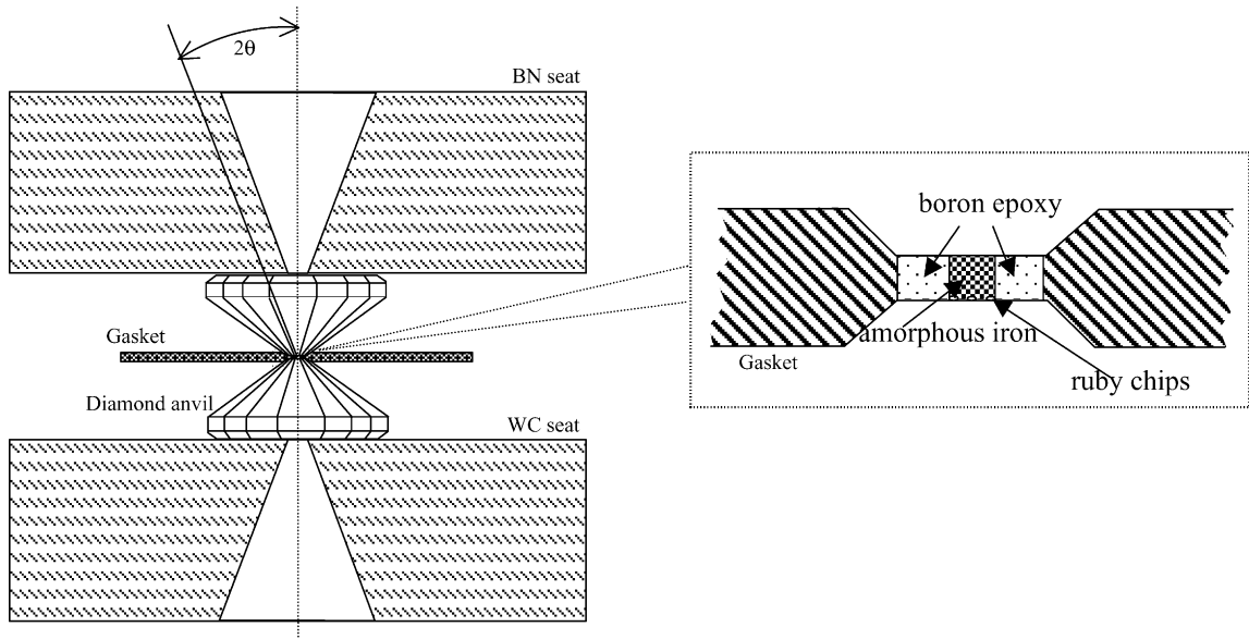
Fig. 1. Schematic of the diamond anvil cell used in this study. One seat is made of boron nitride for a large X-ray access opening. Enlarged figure shows the amorphous-boron insert gasket configuration, which helps in increasing the sample thickness and in performing proper background subtraction.
