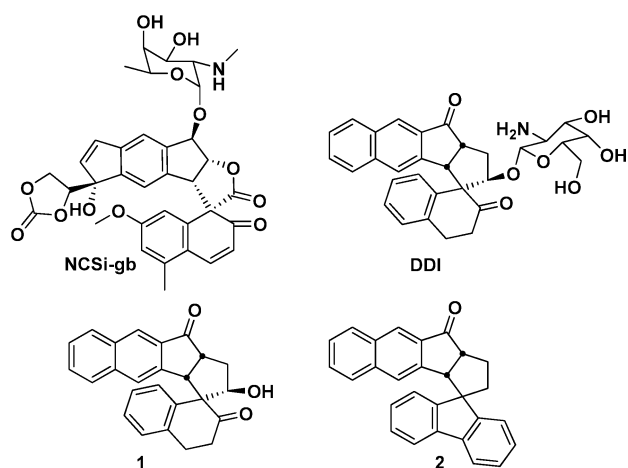
Figure 1. Spirocyclic compounds for RNA-binding studies.
